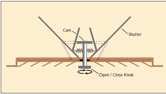
CAM OPERATED OPENING AND CLOSING MECHANISM.
